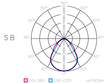
light distribution DOWN
