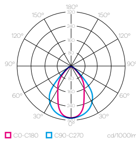
light distribution DOWN MPRM
