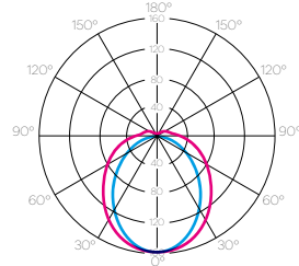
light distribution JET OUT
