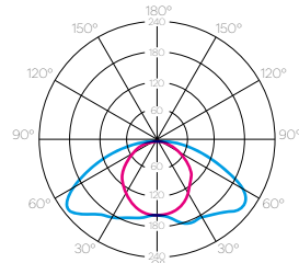
light distribution DOWN OPAL
