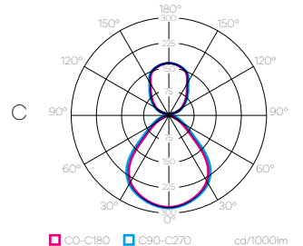
light distribution UP & DOWN
