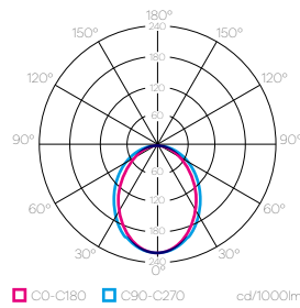
light distribution DOWN OPAL
