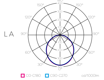
light distribution UP & DOWN
