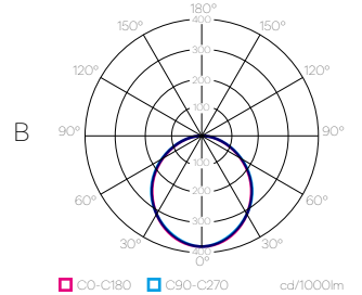
light distribution DOWN
