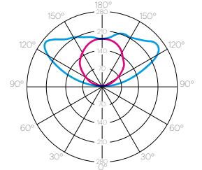
light distribution UP
