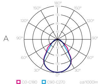
light distribution DOWN
