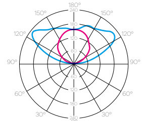
light distribution UP OPAL
