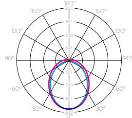
light distribution MID JET
